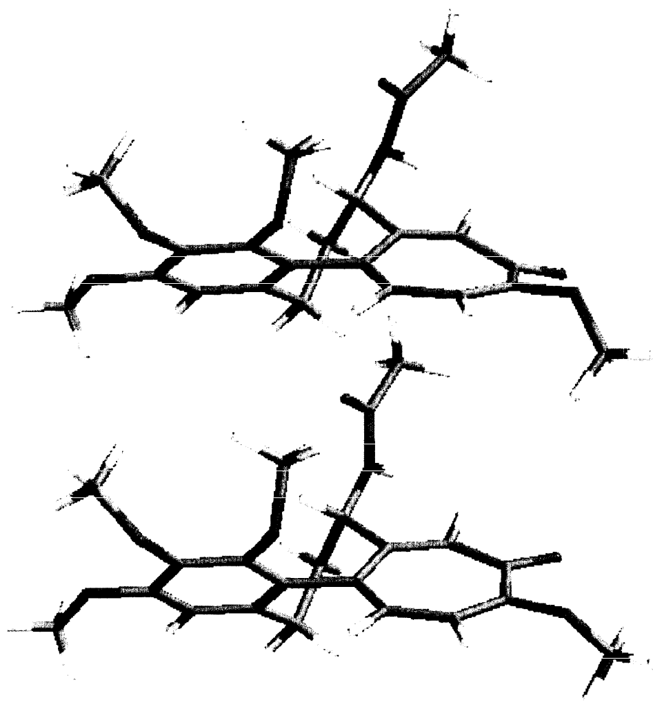
Figure 4. Calculated least-energy conformation for colchicine (top) and its radical anion (bottom)
