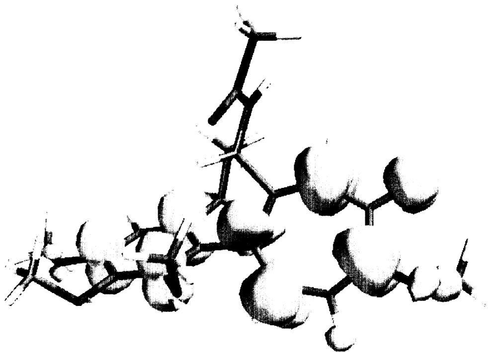
Figure 3. Electron spin density surfaces at 0.002 \text{ e/au}^3 for the colchicine radical anion ( 1r )
