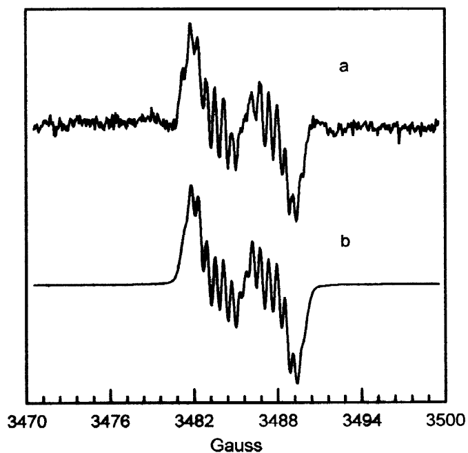
Figure 2. EPR spectrum of deuteriated colchicine ( 4 ) in DMF solution at r.t.: a) experimental spectrum, b) simulated spectrum
