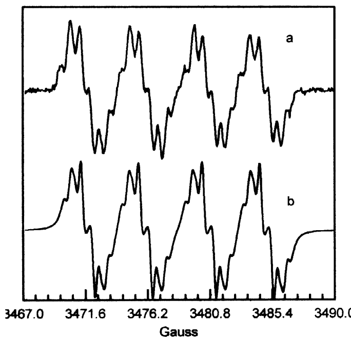
Figure 1. EPR spectrum of colchicine radical anion 1r obtained from cathodic reduction of colchicine ( 1 ) in DMF solution at r.t.: a) experimental spectrum, b) simulated spectrum
